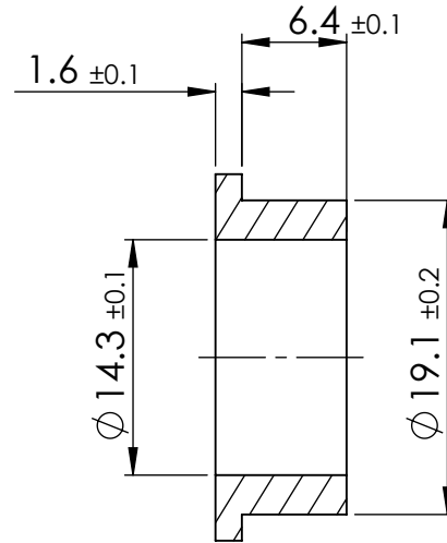
SECTION Y-Y
